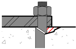
Anchor Bolt Steel ( Vsa )
