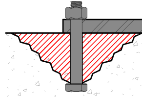
Concrete Breakout ( Ncb )
