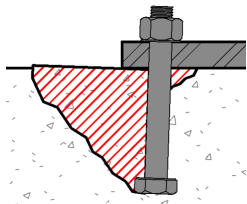
Anchor Bolt Pryout ( Vcp )
