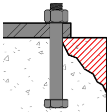
Concrete Breakout ( Vcb )
