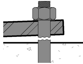
Anchor Bolt Steel ( Nsa )
