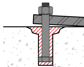
Anchor Bolt Pullout ( Npn )
